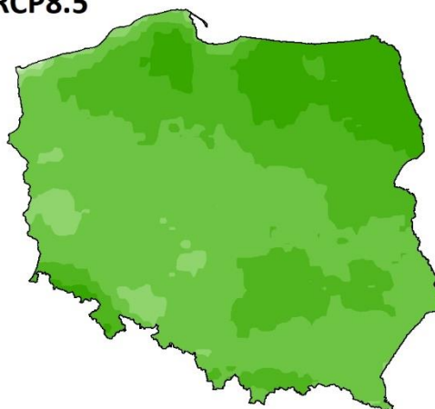
RCP8.5
